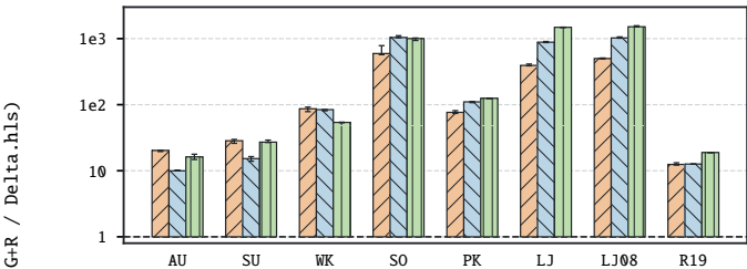
(a) Dynamic algorithms, complete graphs
