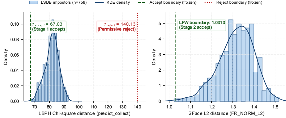
Fig. 3. Histograms and KDE curves of La Salle DB1 clean-impostor scores with frozen LFW operating points overlaid.
