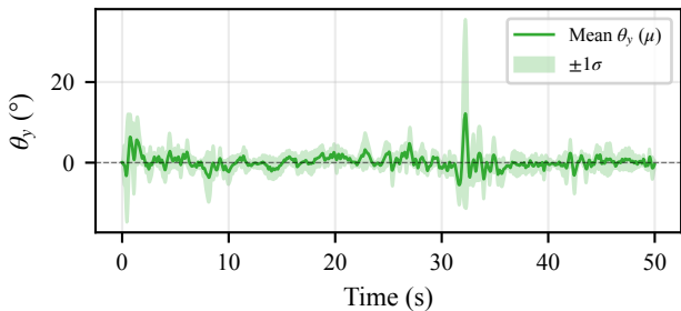
(c) PID + residual RL (trained r \leq 0.2 ) (std=3.6°, max=52.7°)
