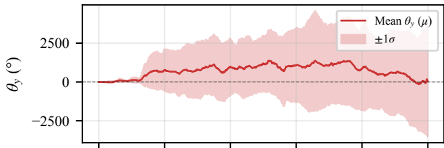
(a) Without attitude control (std=2103.3°, max=5497.7°)
