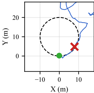
(a) Without attitude control ( \bar{e} = 24.35 m)
