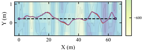
(c) PID + residual RL ( \bar{e} = 0.26 m)
