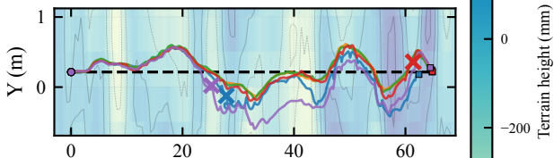
(b) Cascaded PID ( \bar{e} = 0.48 m)
