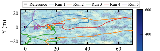
(a) Without attitude control ( \bar{e} = 36.48 m)
