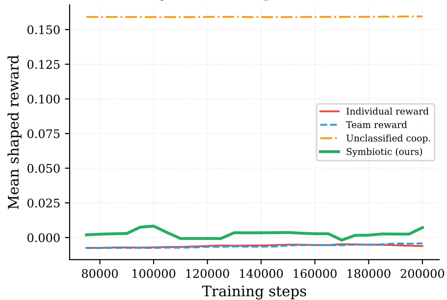
Symbiotic Shaped Reward
