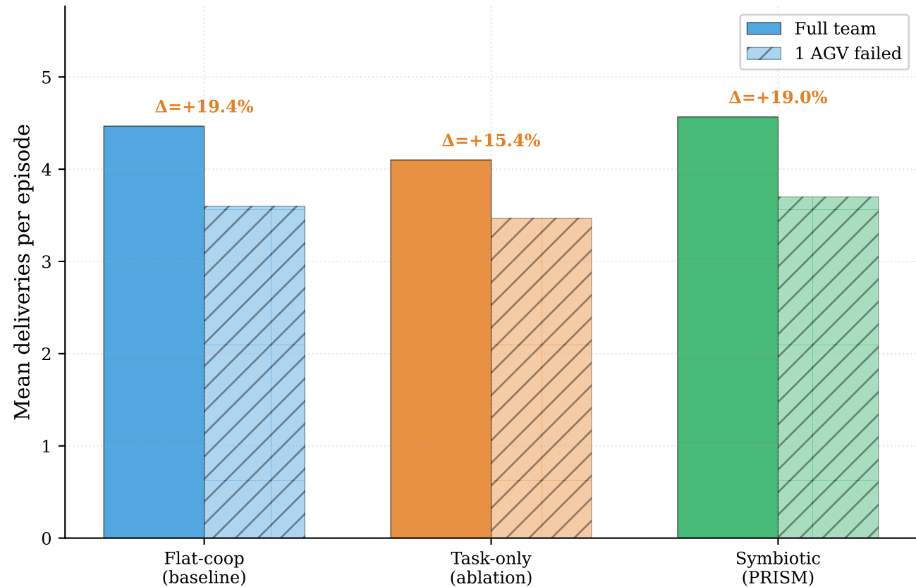
Fig. — Team Resilience Under Agent Failure (lower drop % = more resilient)
