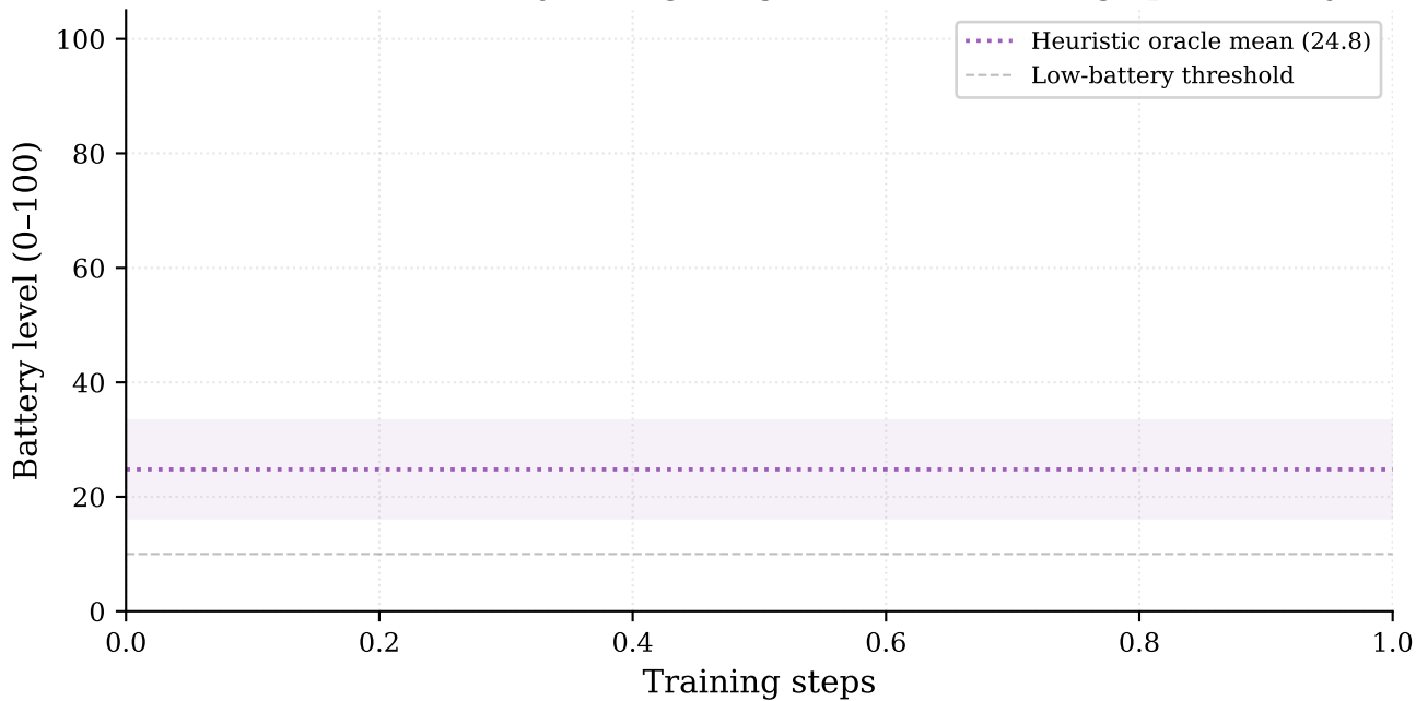
Fig 9 — Battery Management: Mean Agent Battery over Training (dashed = min battery; rising = agents learn to charge proactively)
