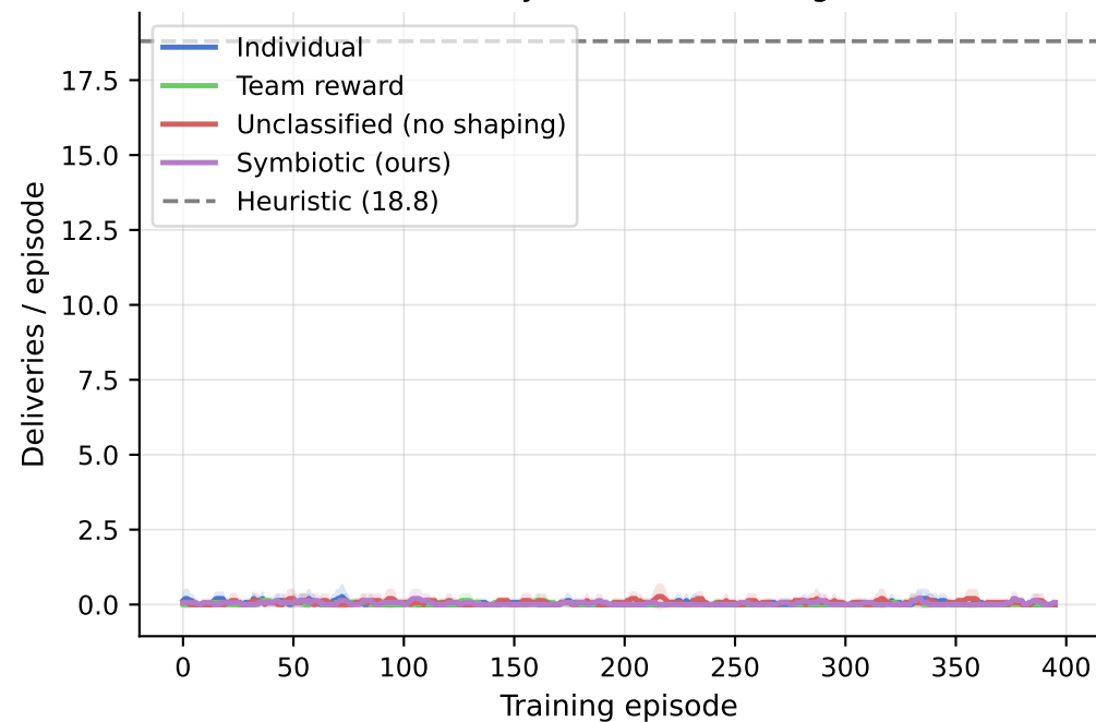
Delivery rate over training
