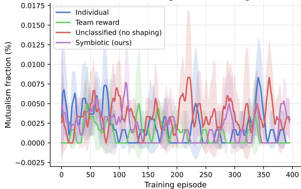
Mutualism emergence over training
