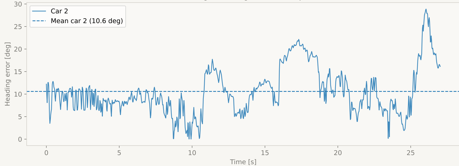
Pose Tracking - Heading Error S1 cooperative
