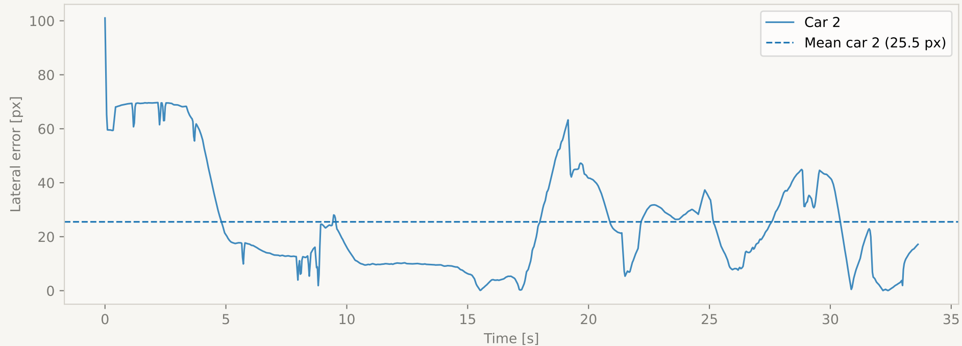
Pose Tracking - Lateral Error S1 cooperative
