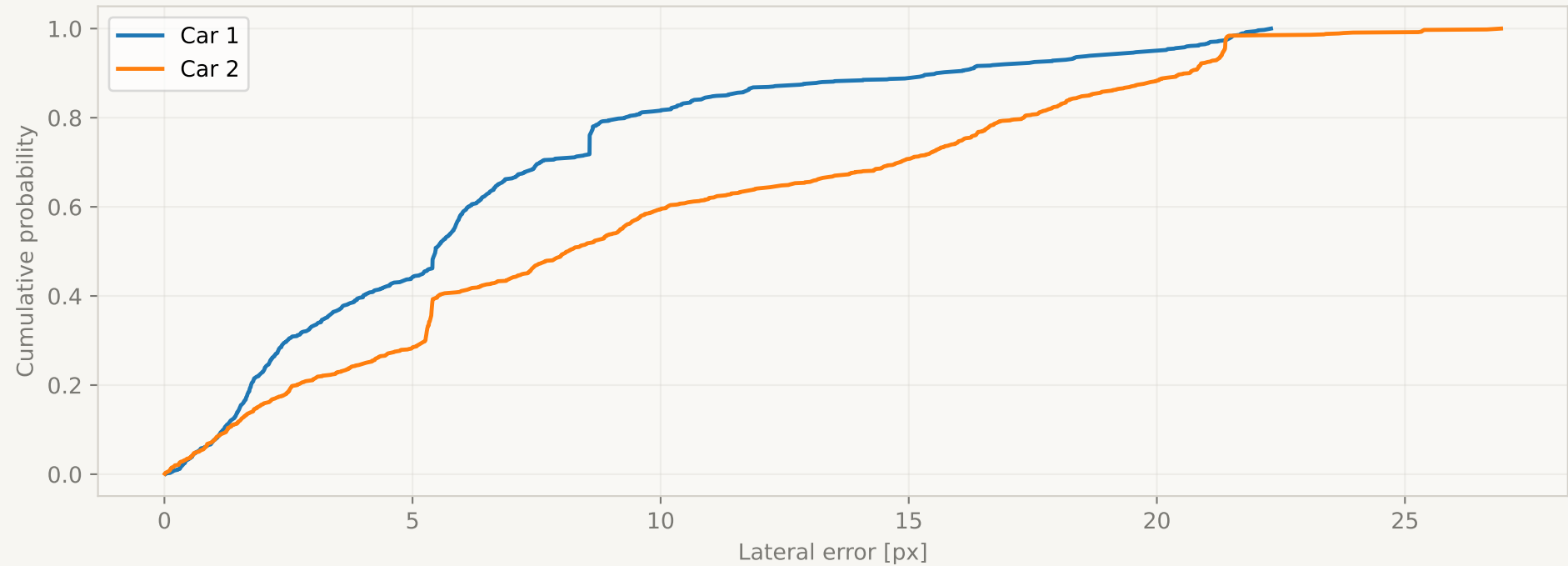
CDF - Lateral Error S2 cooperative
