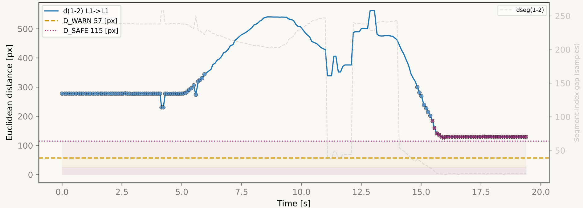
Car-to-Car Distance - Same-Lane S3 cooperative
