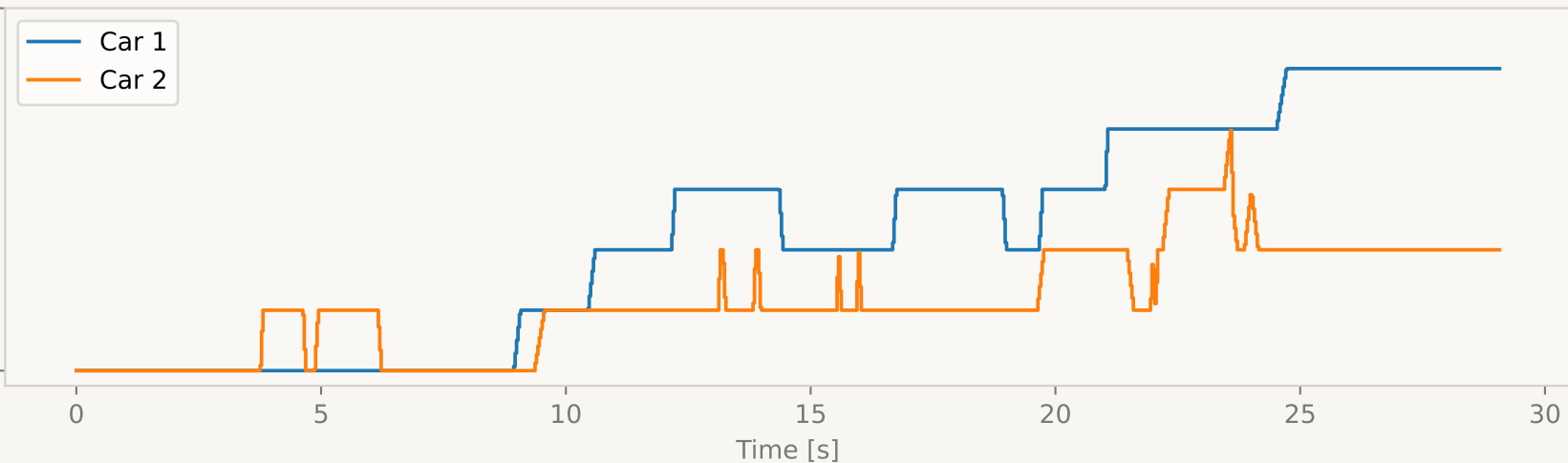
Emergency Stop Active Frames S3 cooperative
