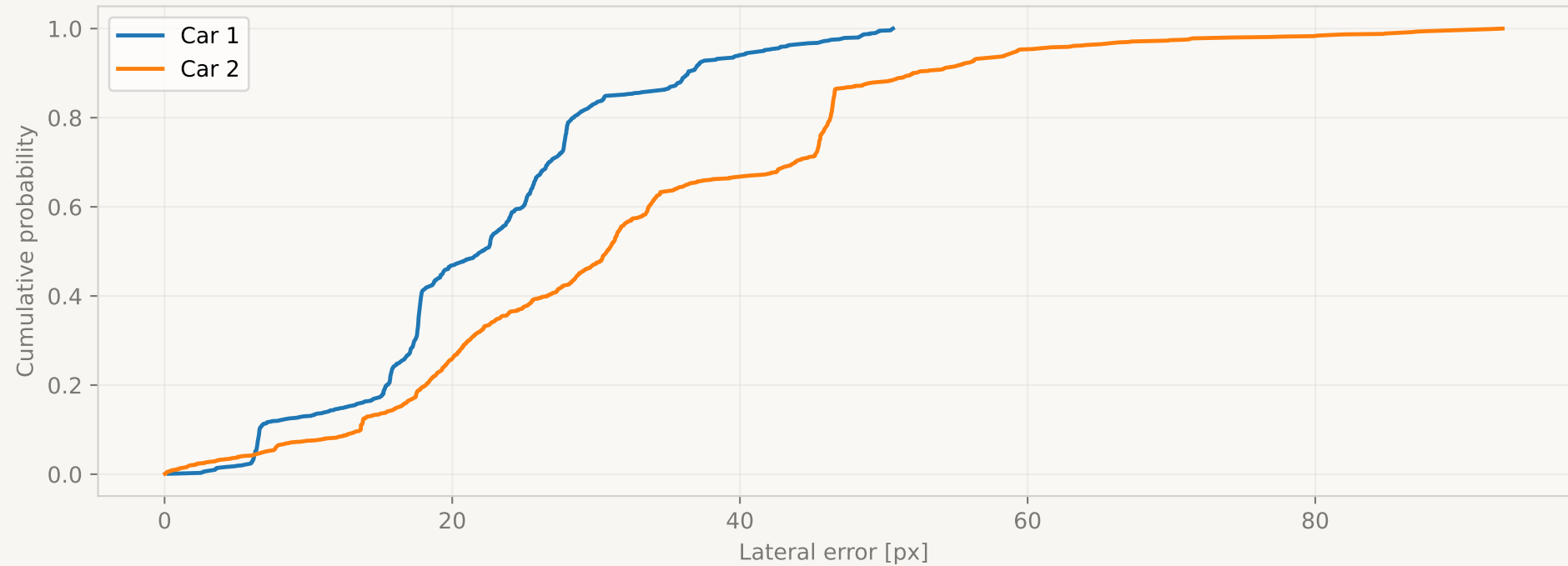
CDF - Lateral Error S3 cooperative
