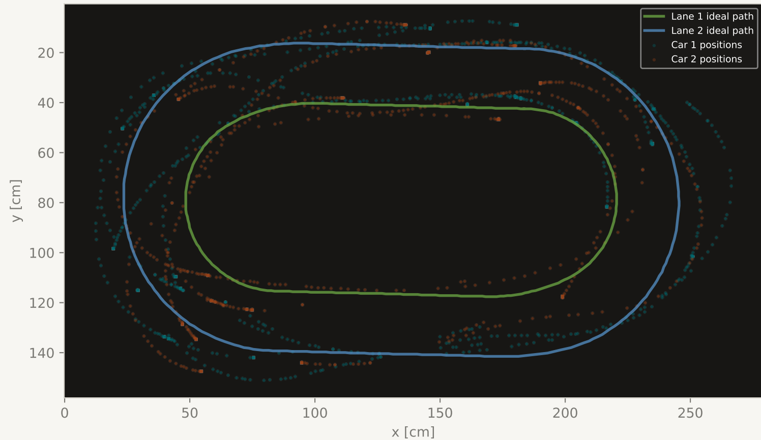
Trajectory Coverage S3 cooperative dFOV=90deg (6 runs averaged)
