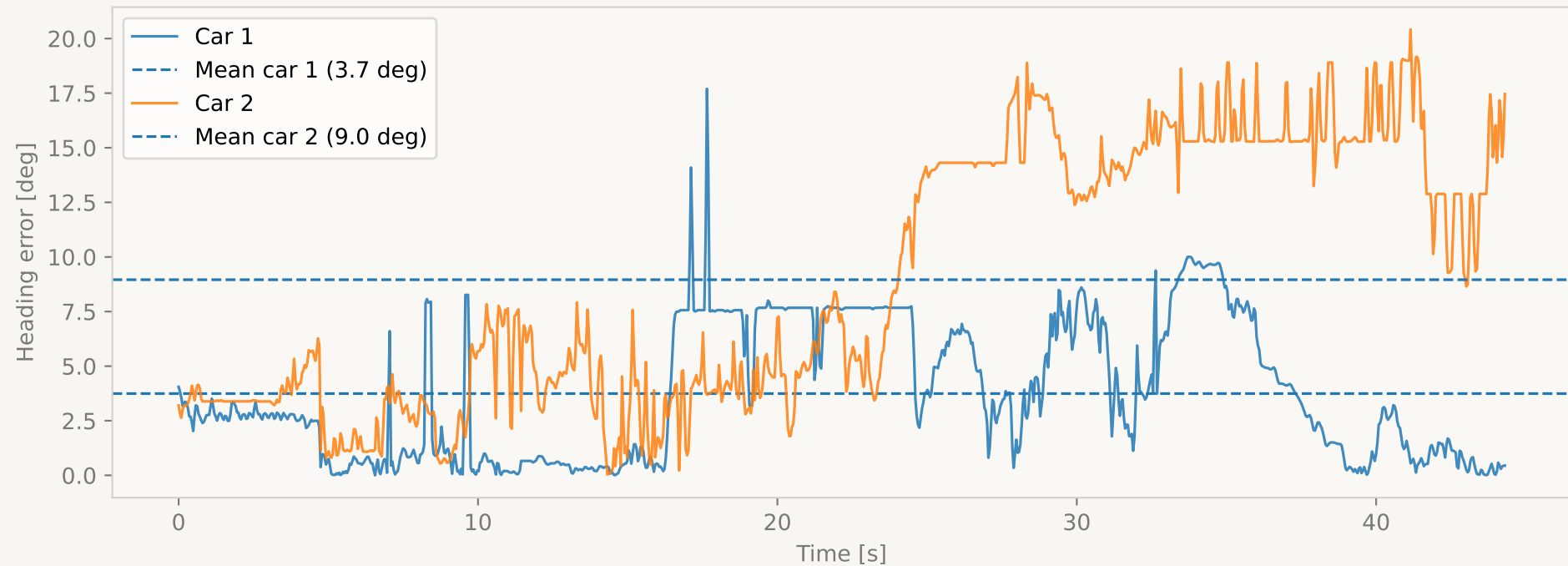
Pose Tracking - Heading Error S3 cooperative
