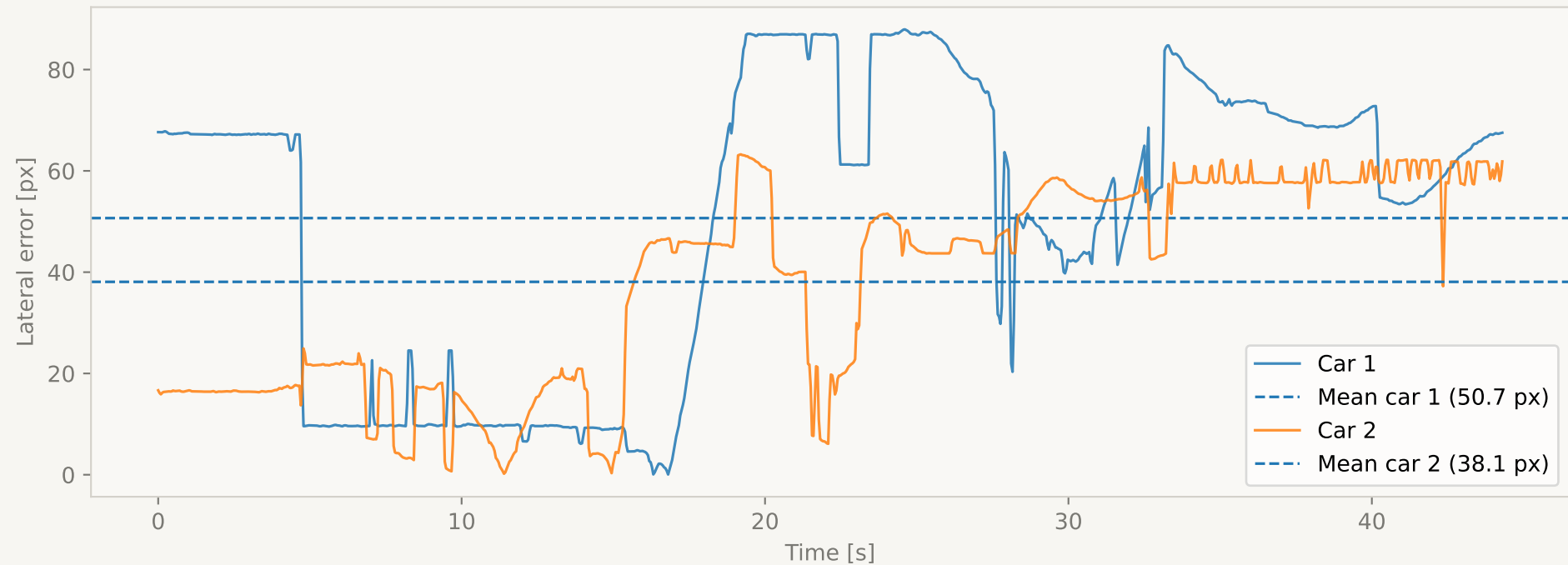
Pose Tracking - Lateral Error S3 cooperative
