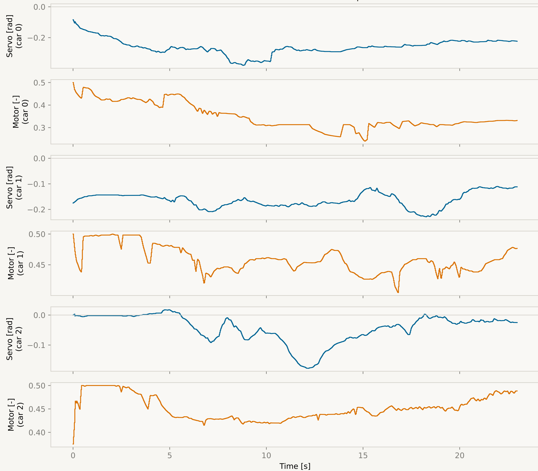
Commands - Servo & Motor S4 cooperative
