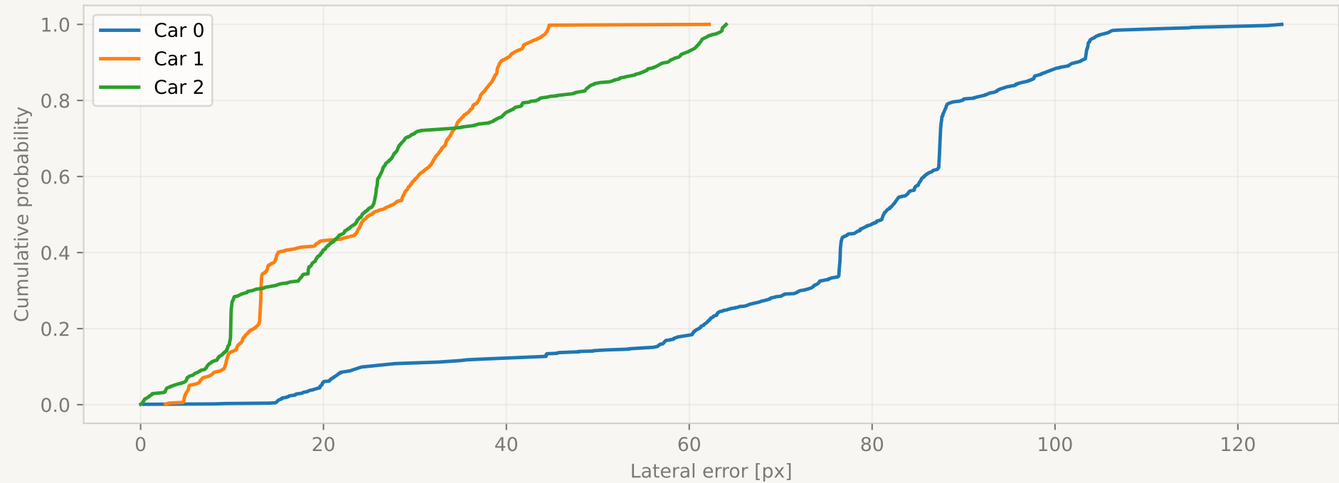
CDF - Lateral Error S4 cooperative
