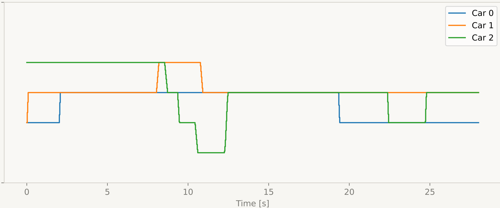
Lane Assignment Over Time S4 cooperative
