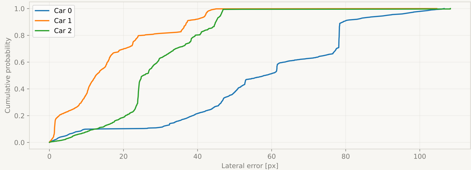
CDF - Lateral Error S4 non_cooperative
