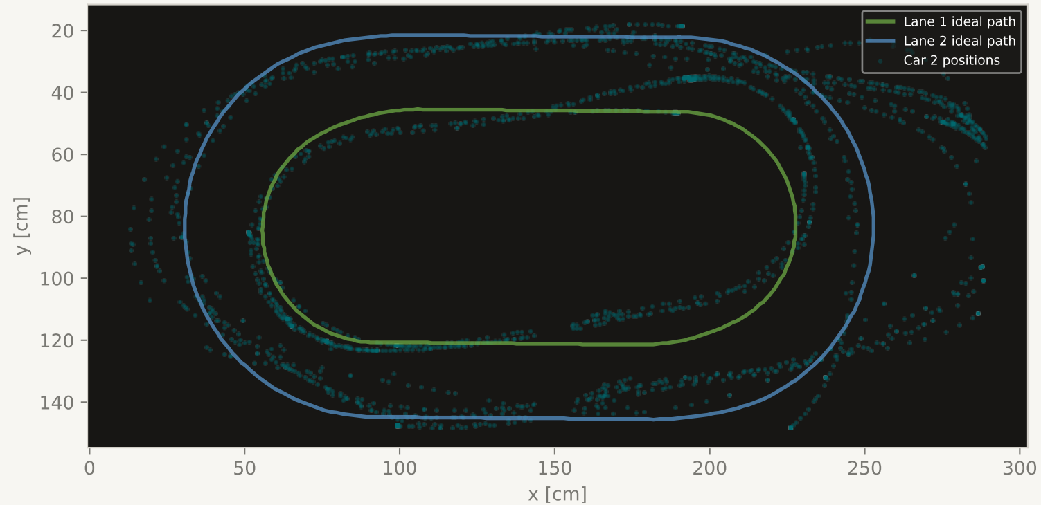
Trajectory Coverage S1 cooperative dFOV=78deg (6 runs averaged)
