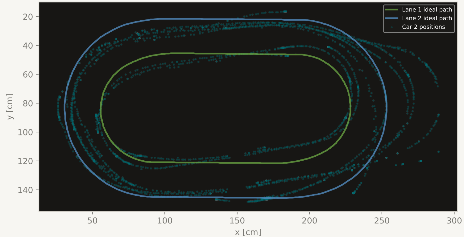
Trajectory Coverage S1 cooperative dFOV=78deg (6 runs averaged)
