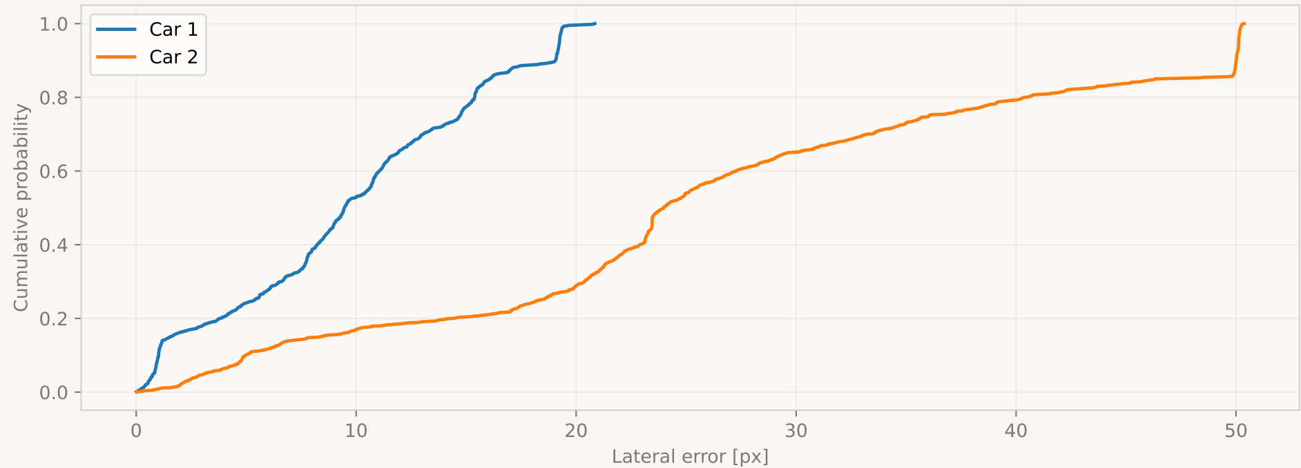
CDF - Lateral Error S2 cooperative
