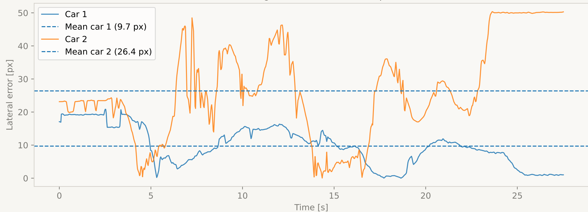
Pose Tracking - Lateral Error S2 cooperative
