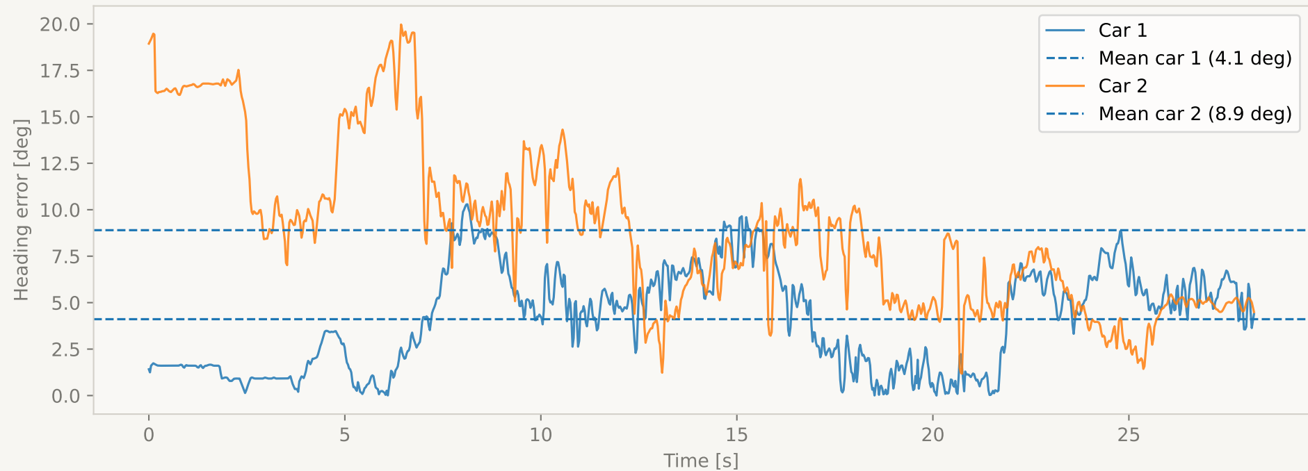
Pose Tracking - Heading Error S2 cooperative
