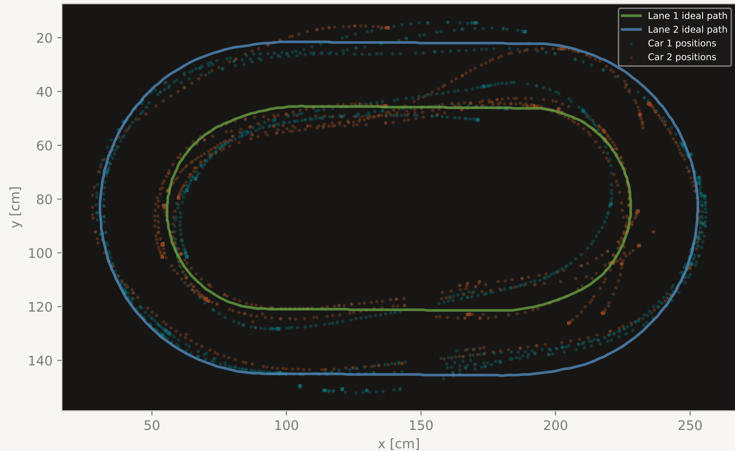
Trajectory Coverage S2 cooperative dFOV=78deg (6 runs averaged)
