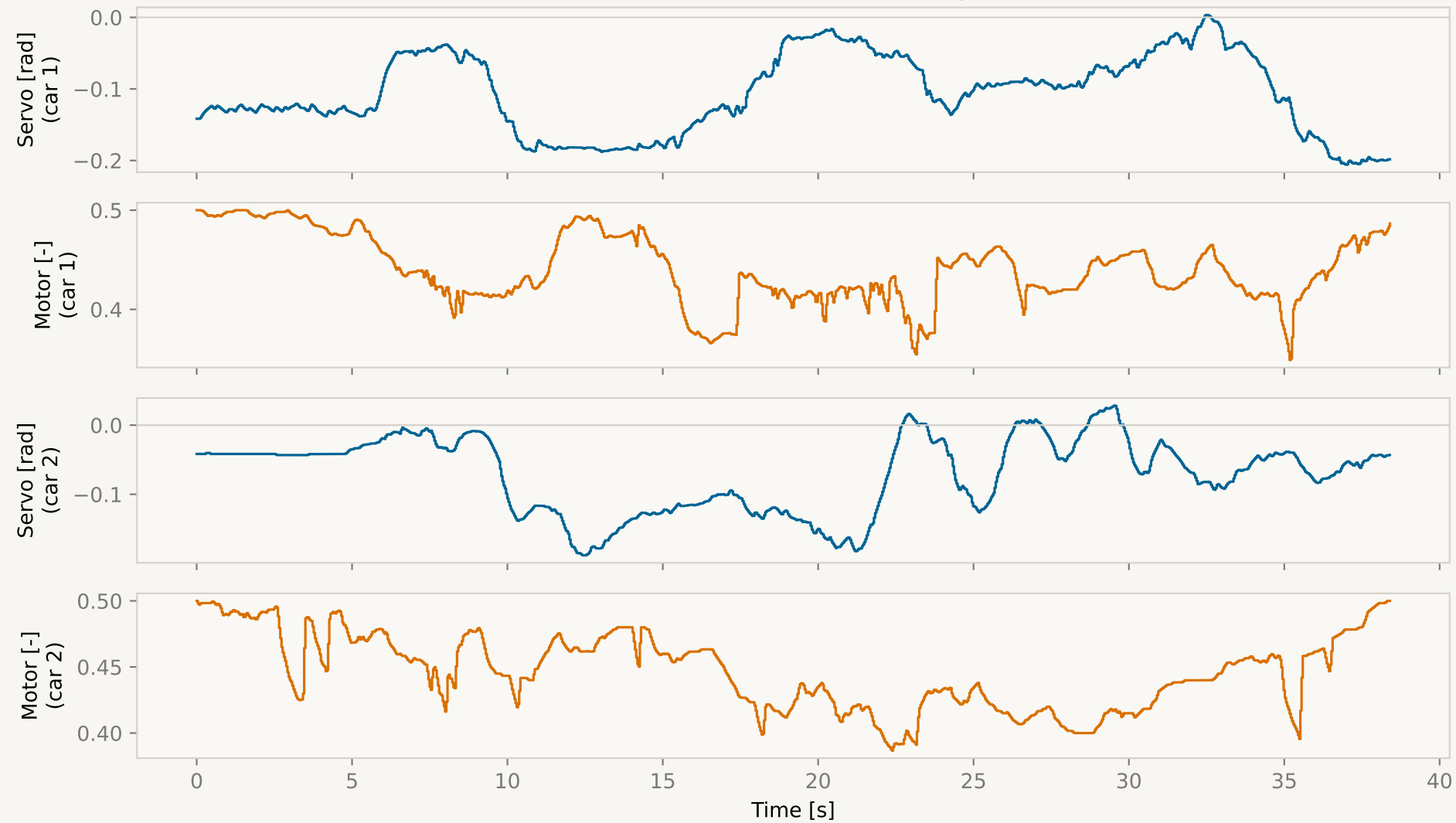
Commands - Servo & Motor S2 cooperative
