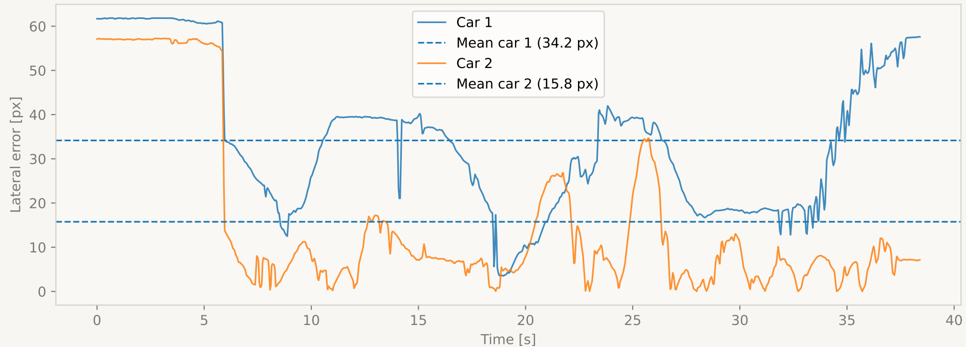
Pose Tracking - Lateral Error S2 cooperative
