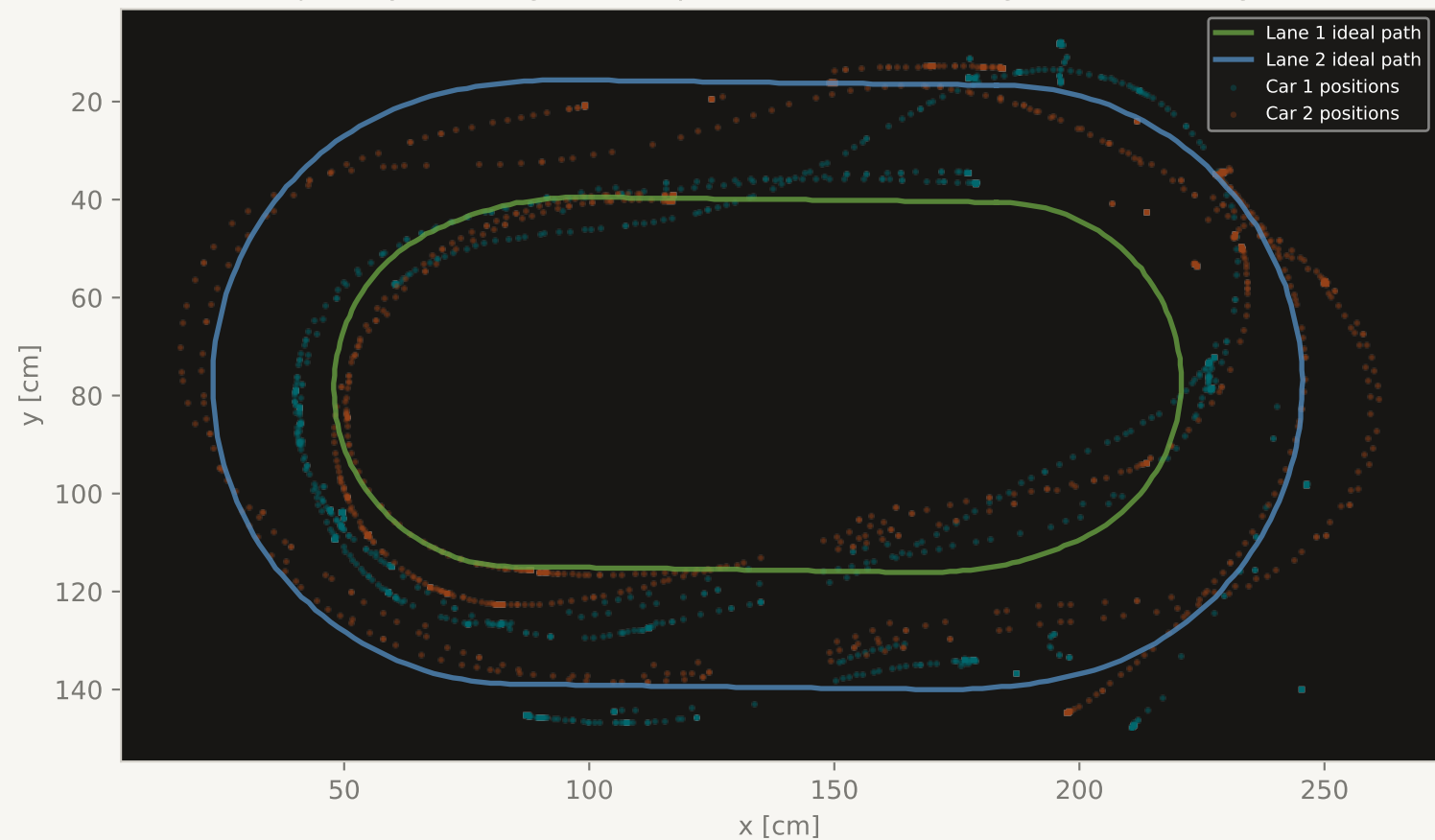
Trajectory Coverage S2 cooperative dFOV=90deg (6 runs averaged)
