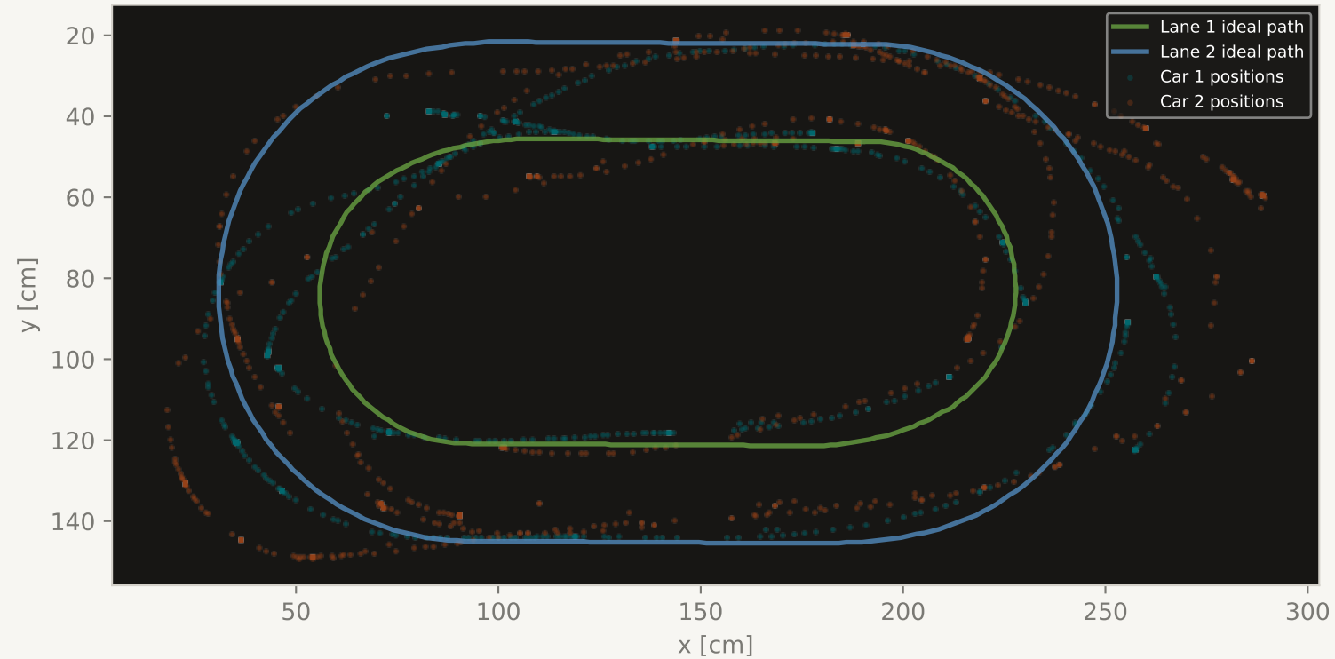
Trajectory Coverage S3 cooperative dFOV=78deg (6 runs averaged)
