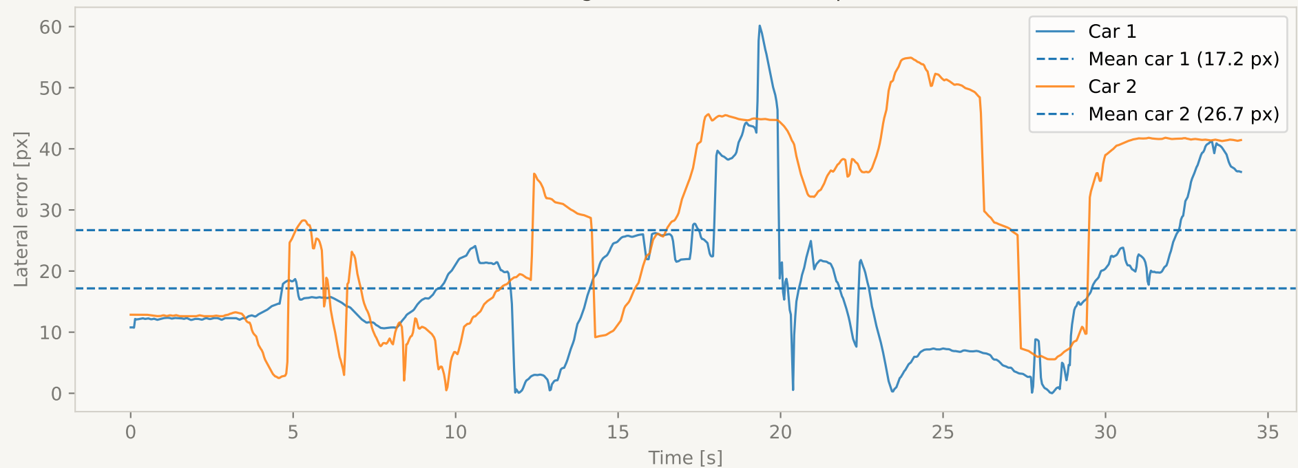
Pose Tracking - Lateral Error S3 cooperative
