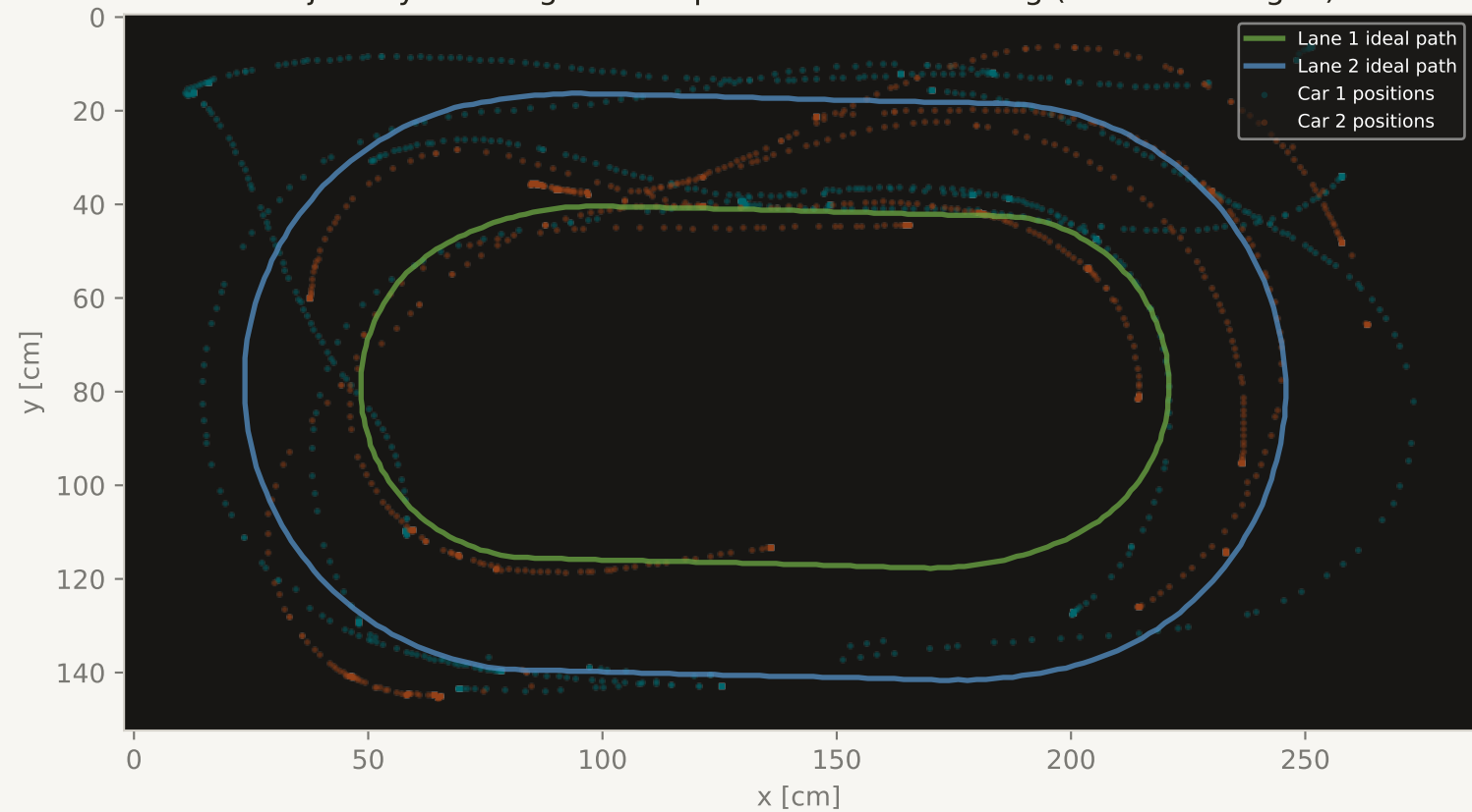
Trajectory Coverage S3 cooperative dFOV=90deg (6 runs averaged)
