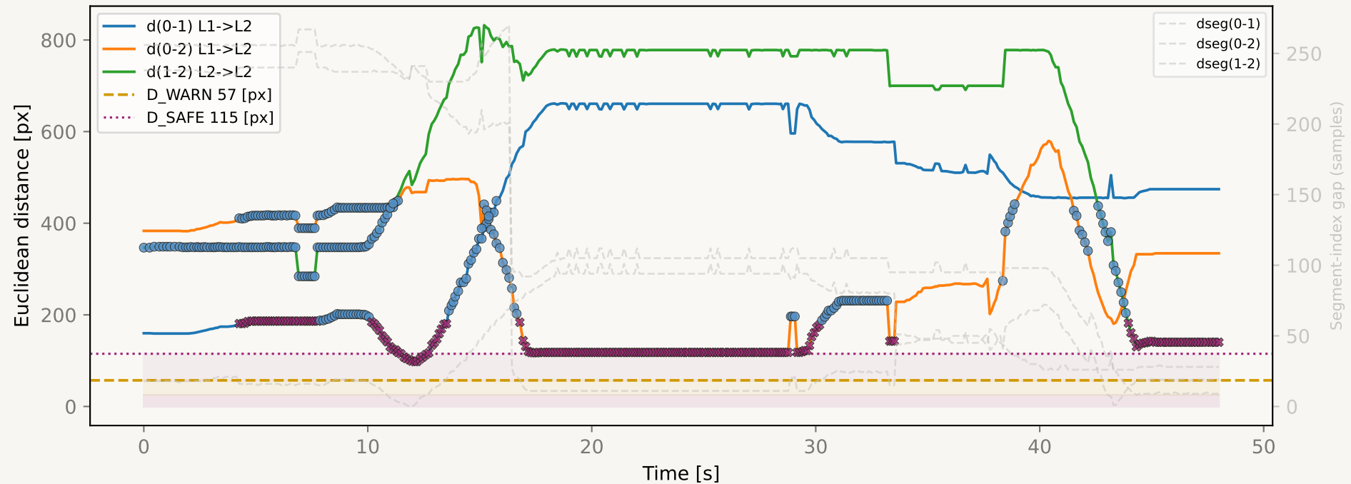
Car-to-Car Distance - Same-Lane S4 cooperative
