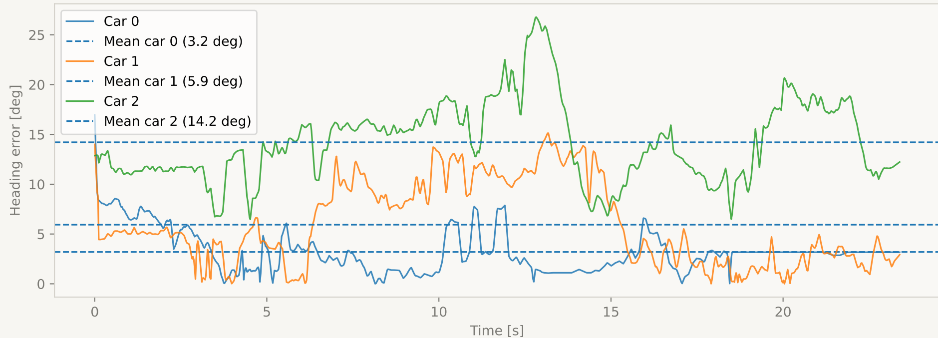
Pose Tracking - Heading Error S4 non_cooperative
