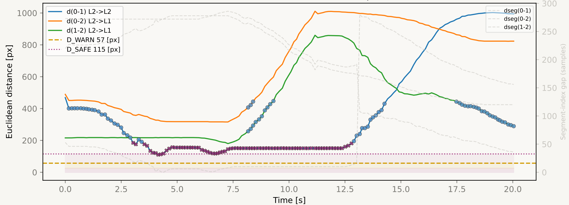
Car-to-Car Distance - Same-Lane S4 cooperative
