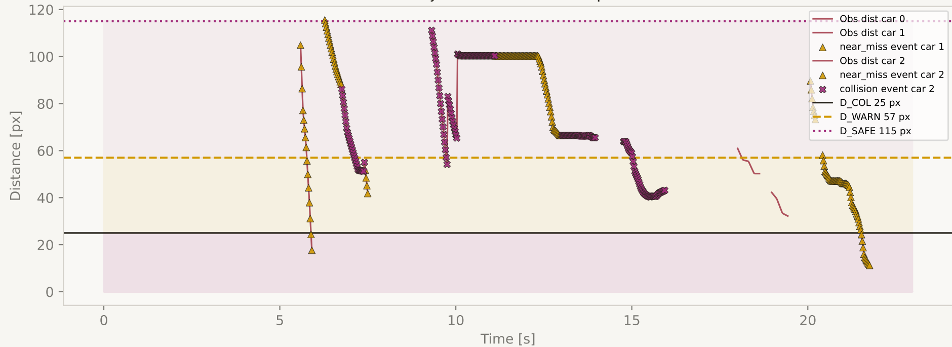
Car-to-Object Distance S4 cooperative
