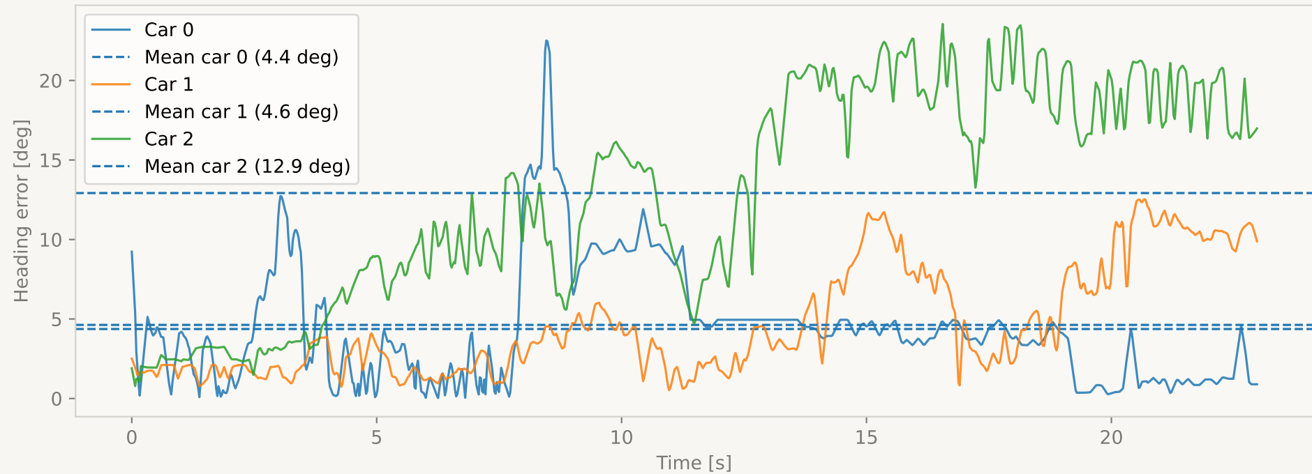
Pose Tracking - Heading Error S4 cooperative
