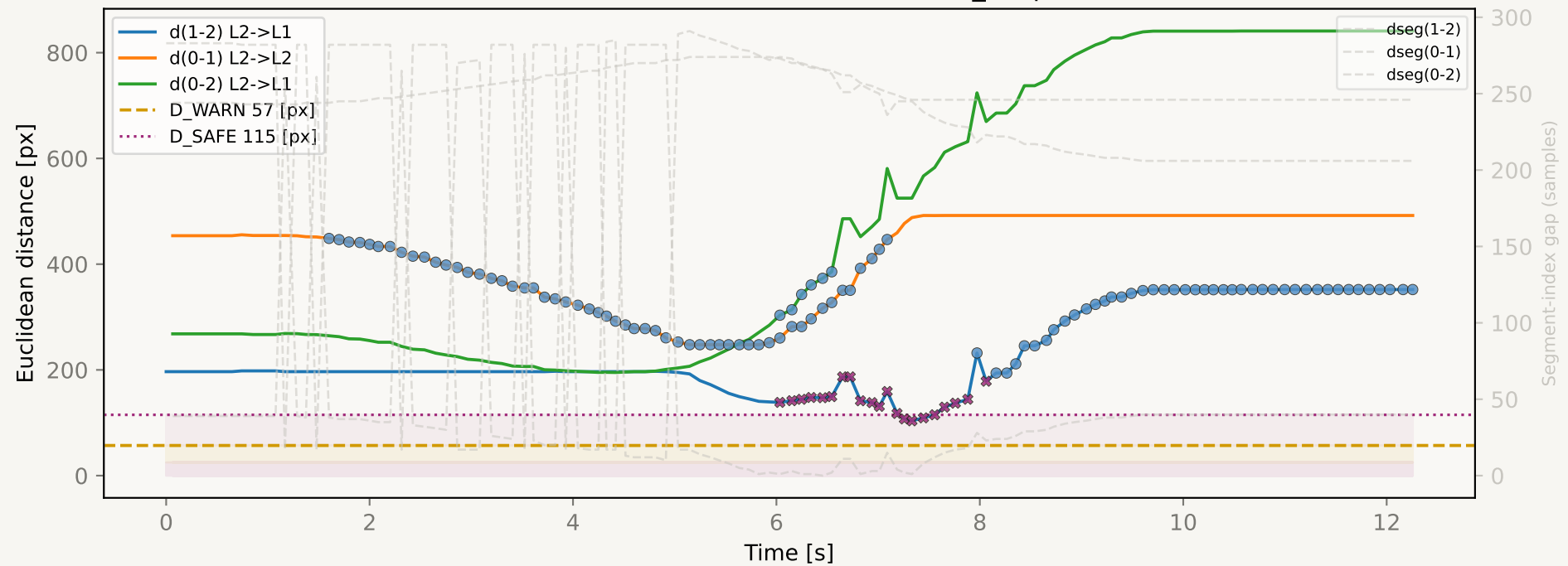
Car-to-Car Distance - Same-Lane S4 non_cooperative
