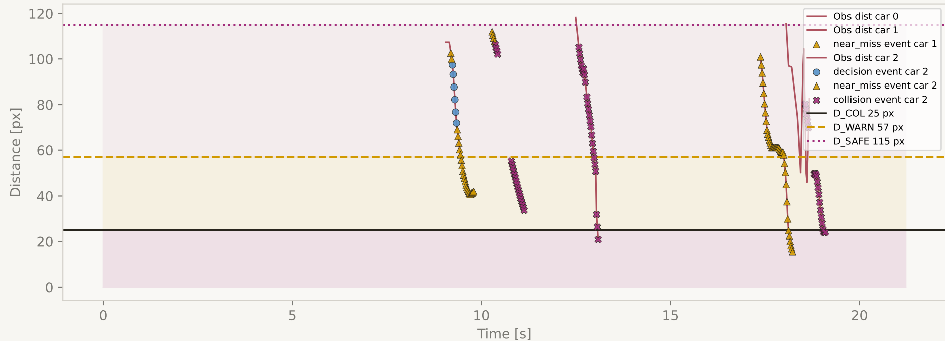
Car-to-Object Distance S4 non_cooperative
