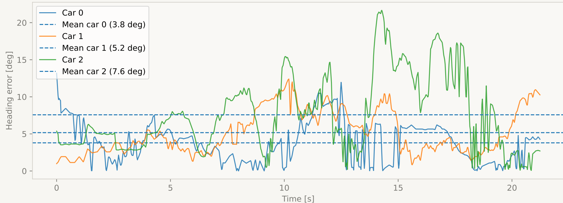
Pose Tracking - Heading Error S4 non_cooperative
