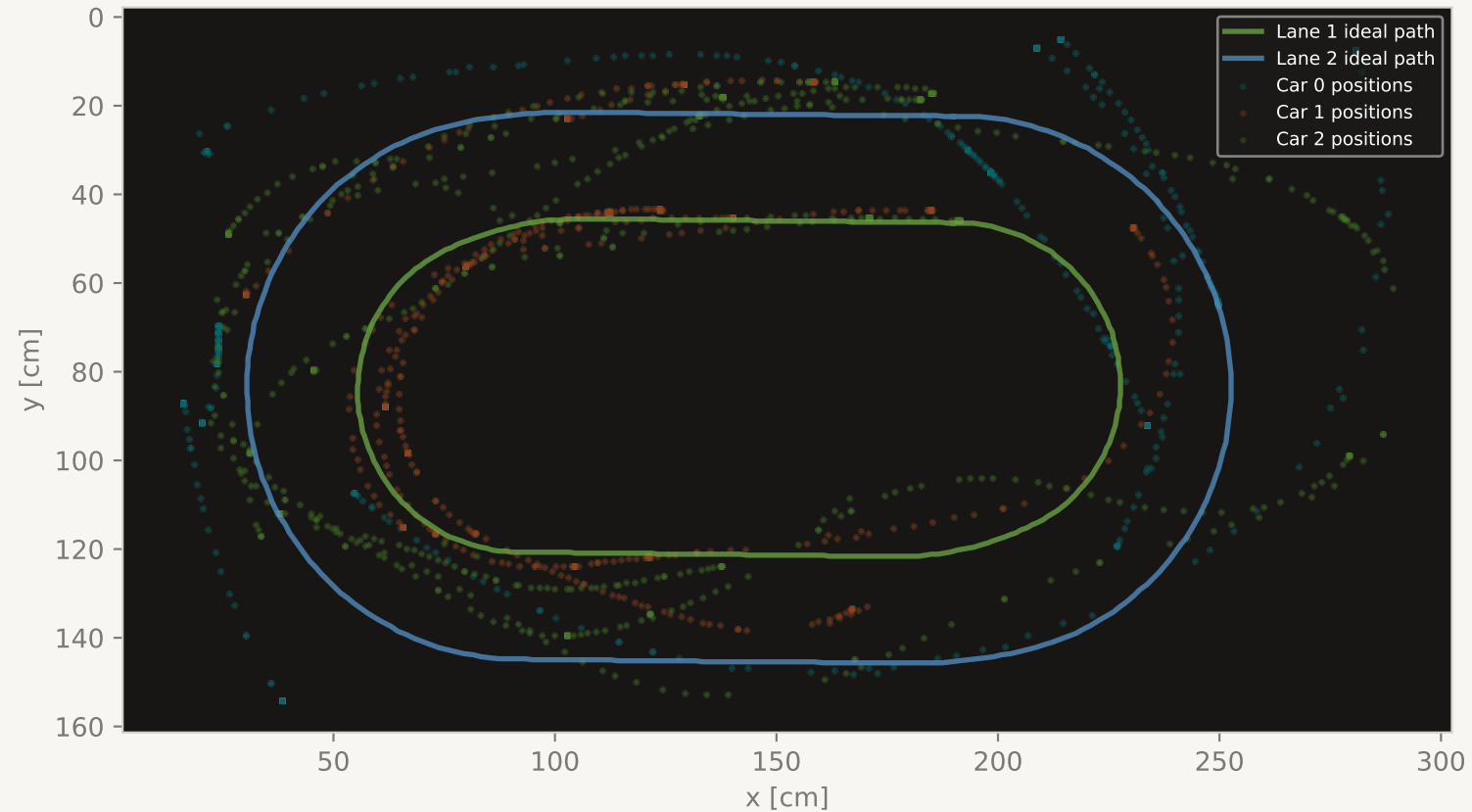
Trajectory Coverage S4 non_cooperative dFOV=78deg (6 runs averaged)
