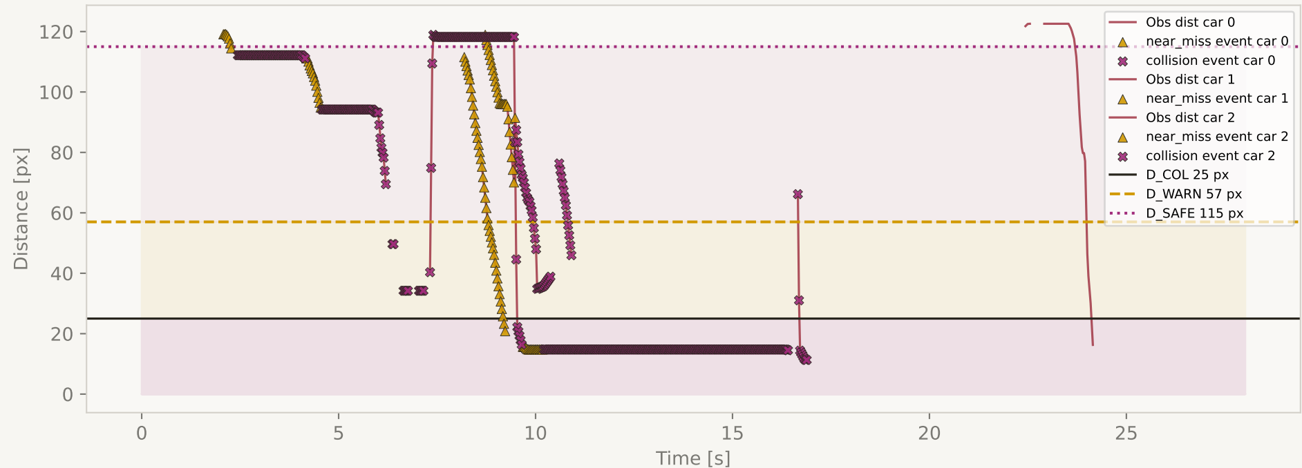
Car-to-Object Distance S4 cooperative
