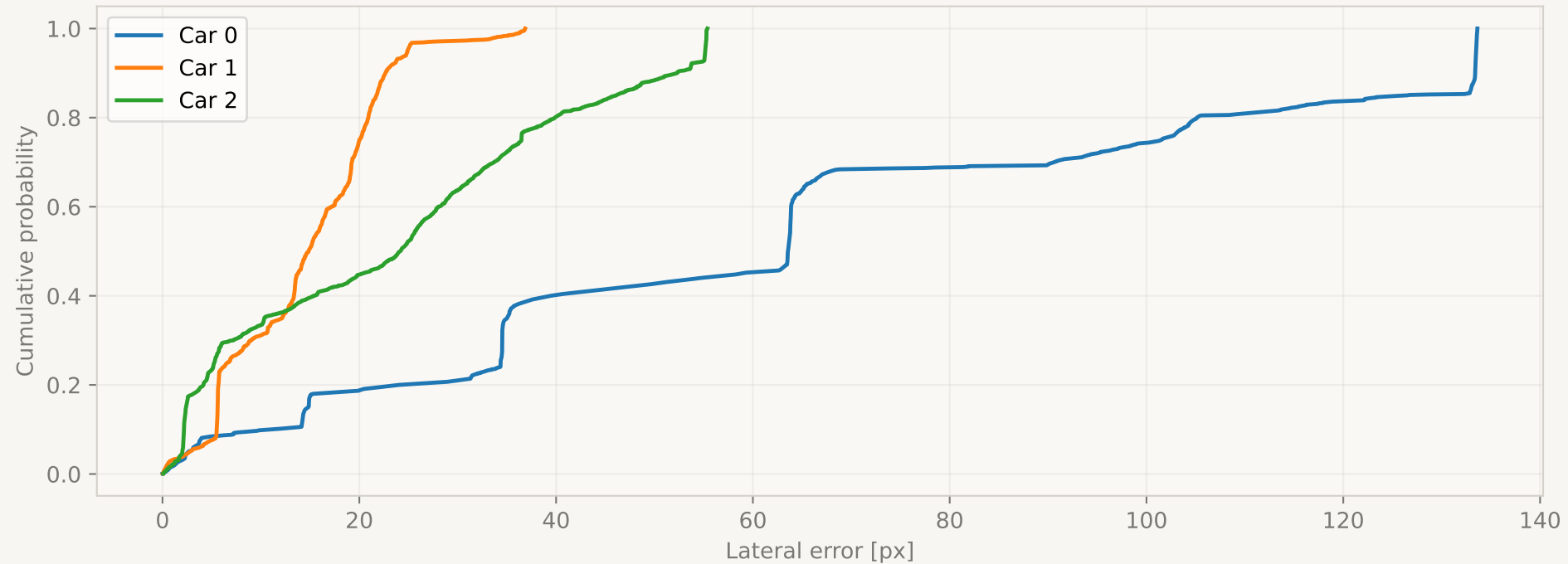
CDF - Lateral Error S4 cooperative
