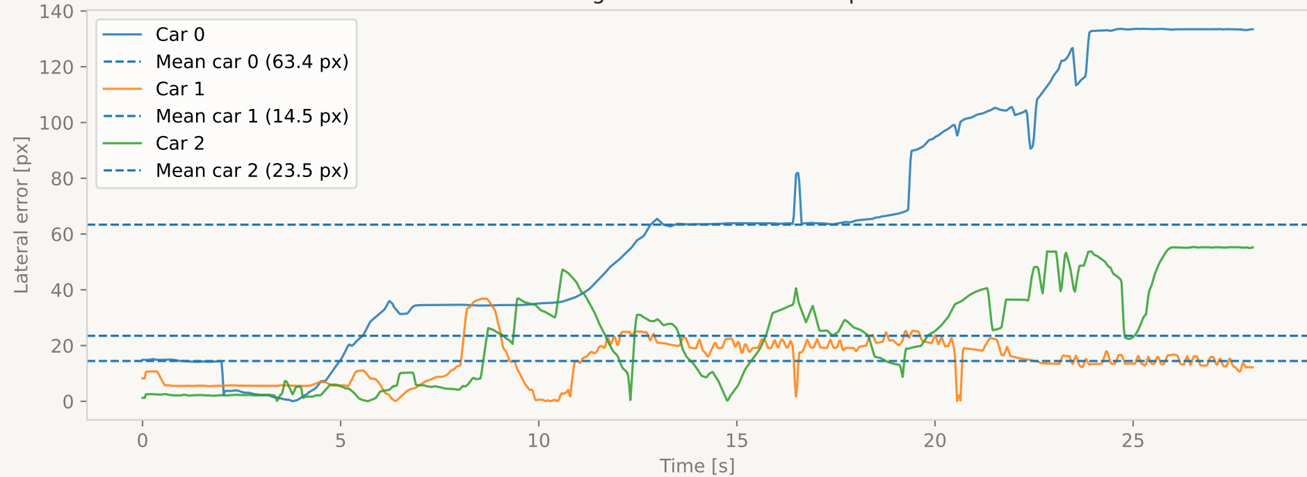
Pose Tracking - Lateral Error S4 cooperative
