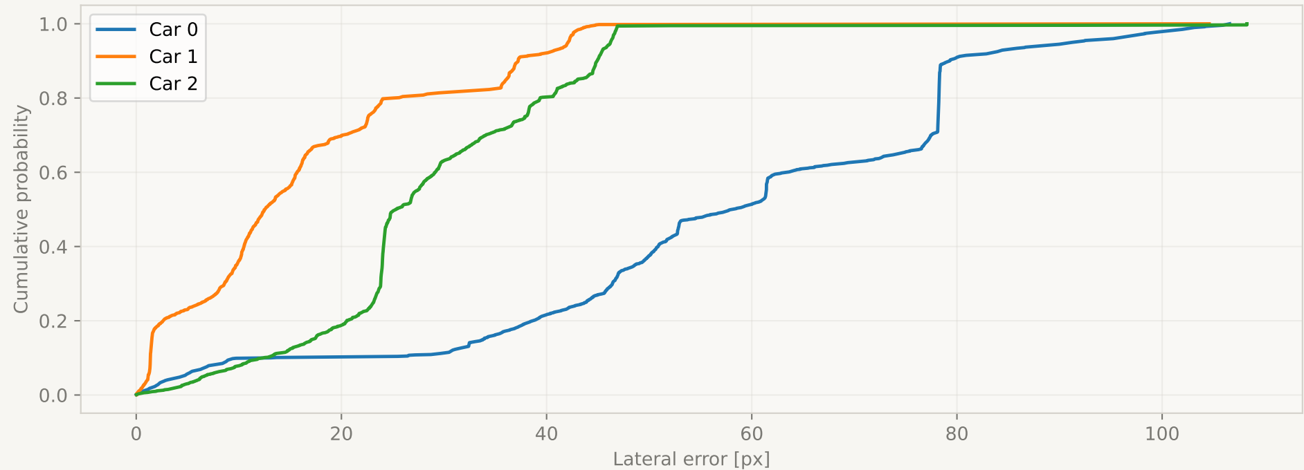
CDF - Lateral Error S4 non_cooperative
