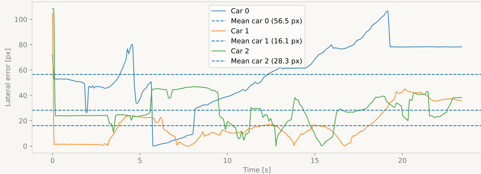
Pose Tracking - Lateral Error S4 non_cooperative
