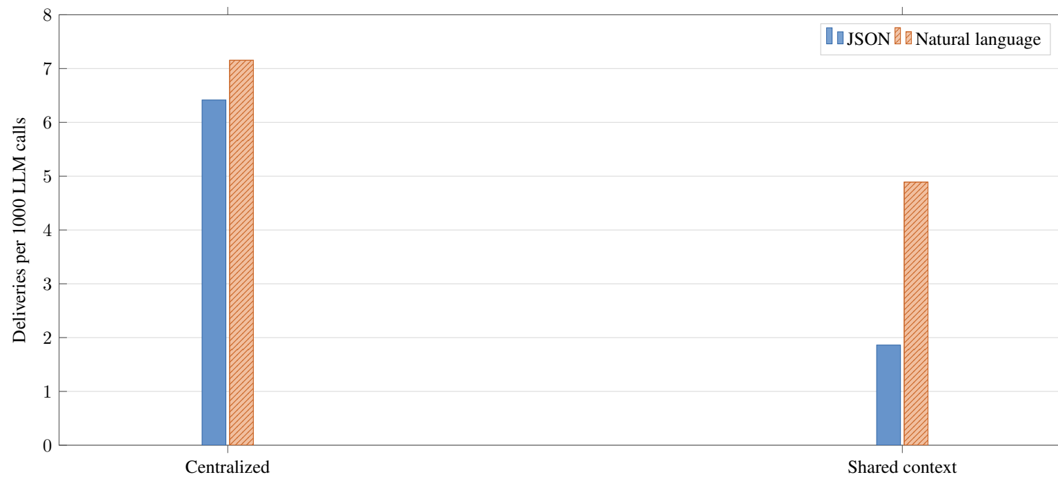
Prompt configuration within each planning architecture
