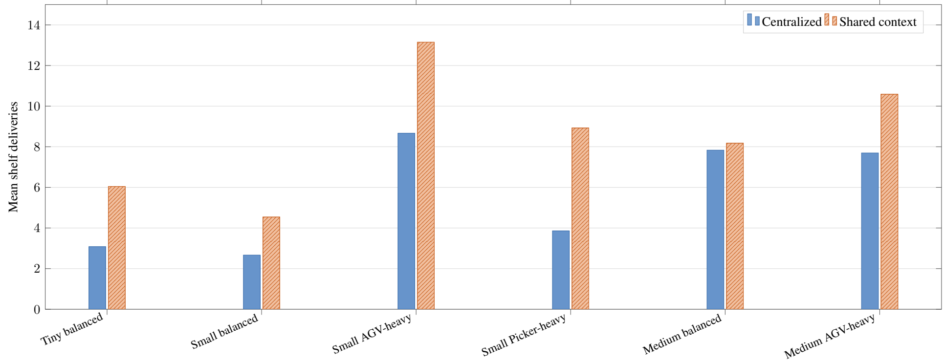
Mean delivery count by planning architecture and scenario
