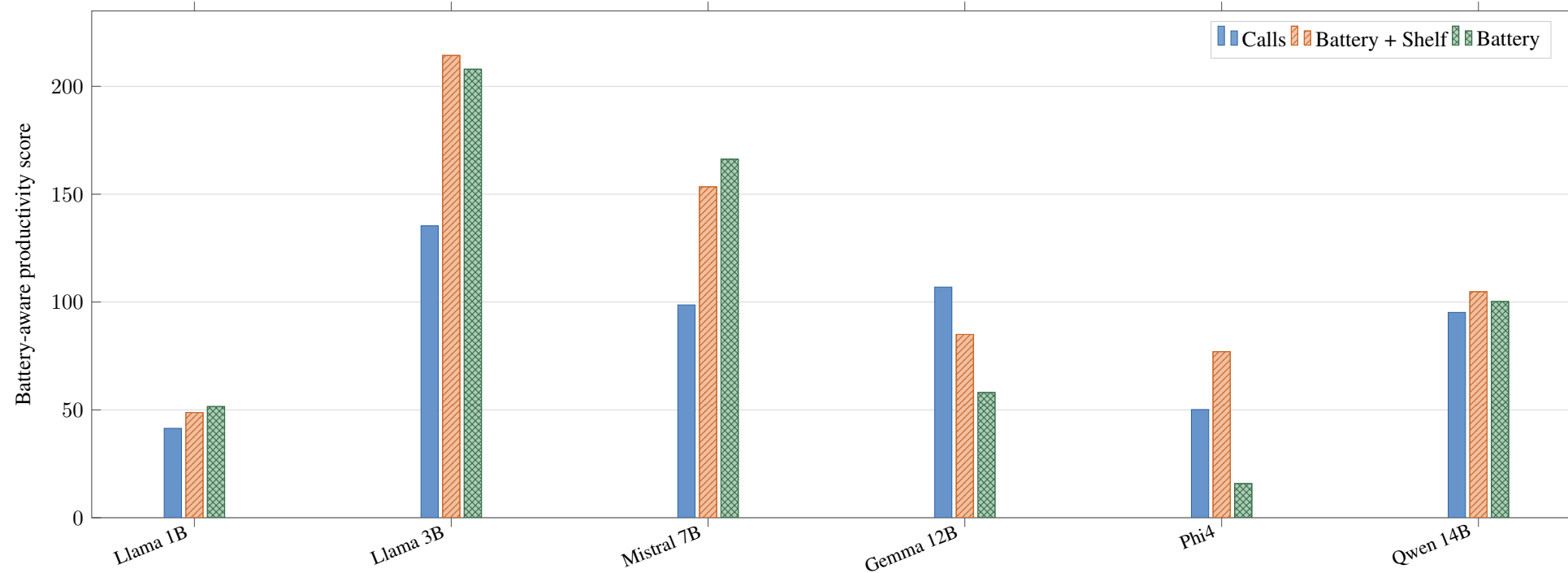
Battery-aware productivity by objective and model
