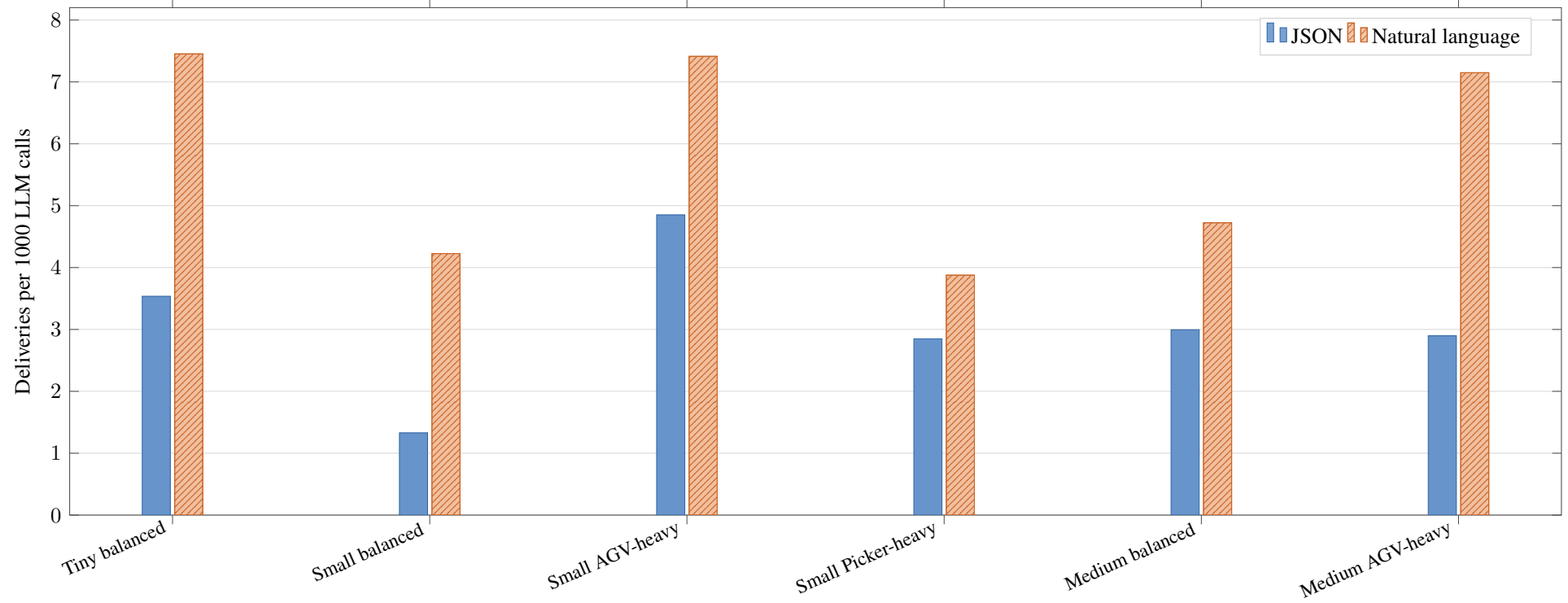
Call-normalised deliveries by prompt configuration and scenario
