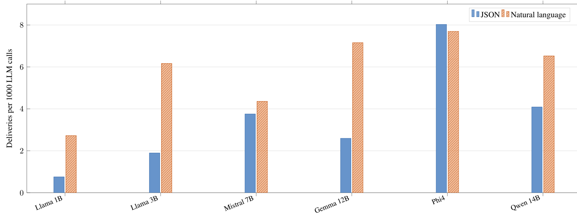
Call-normalised deliveries by prompt configuration and model
