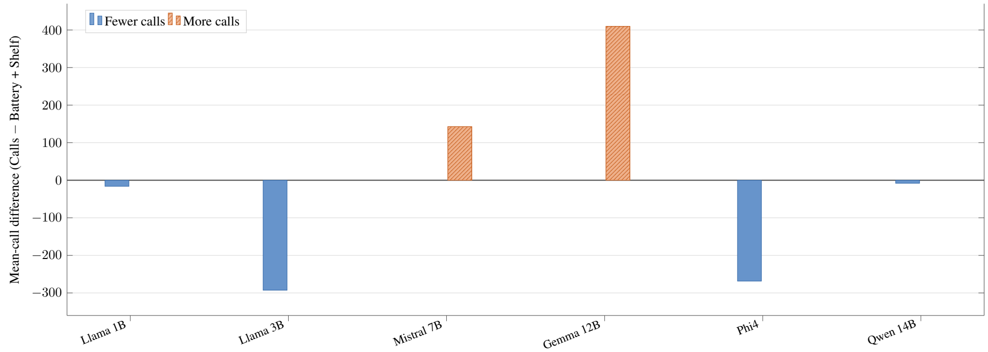
Change in LLM calls under the call-reduction objective
