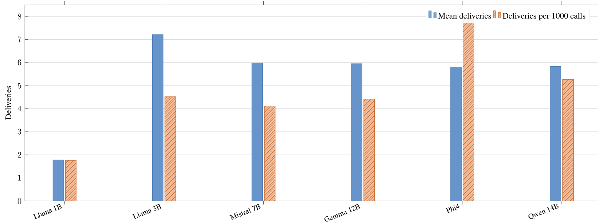
Matched delivery performance by model
