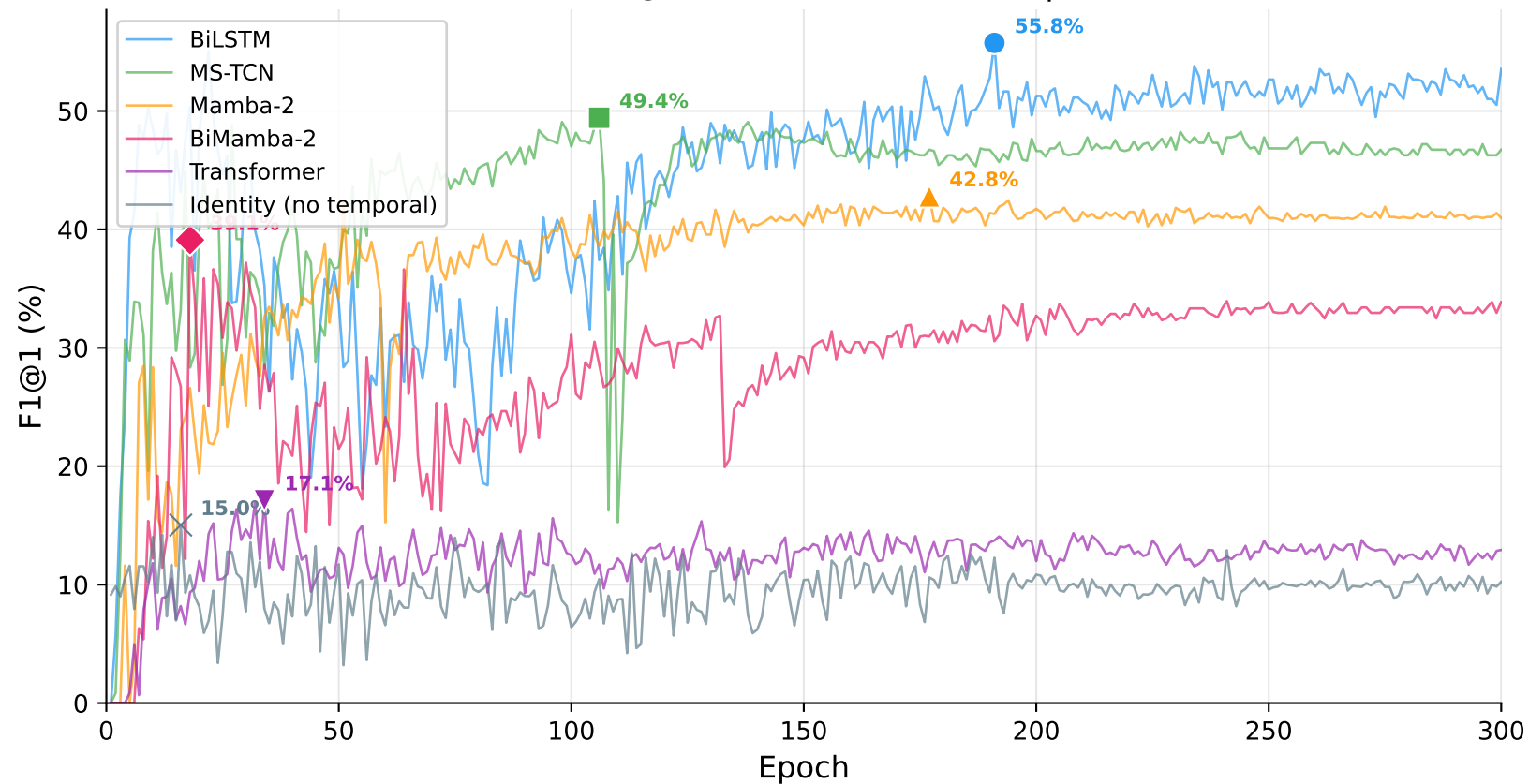
Hit Detection F1@1 ( \pm 1 frame) — All Temporal Heads
